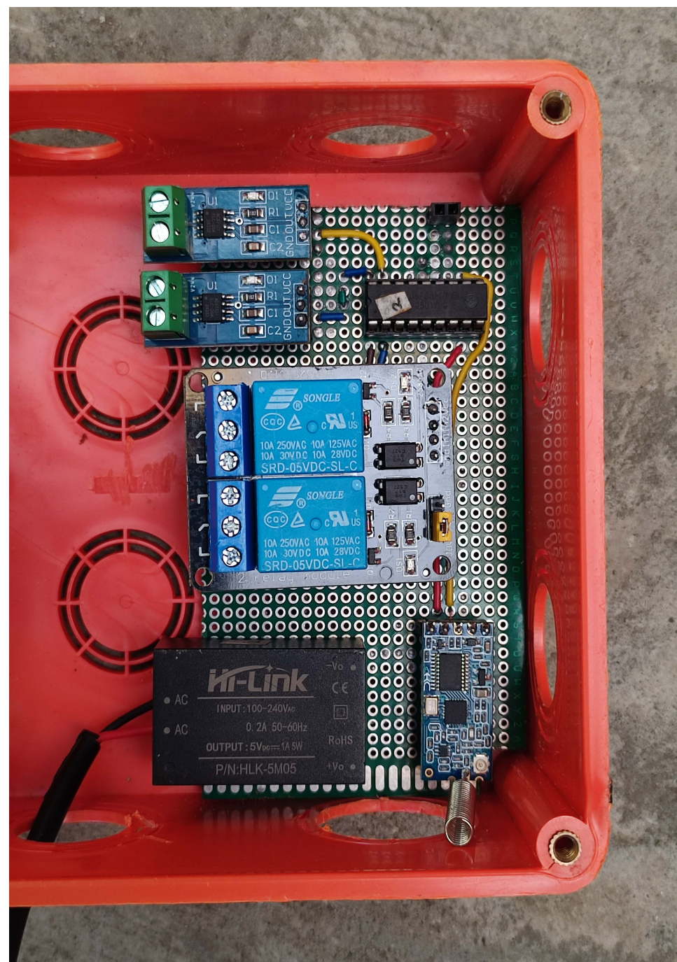
Full Circuit
