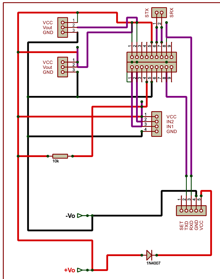
Full Circuit
